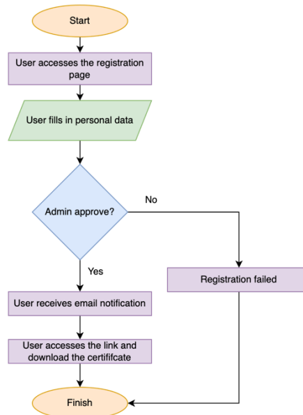
Figure 4. Registration flow
