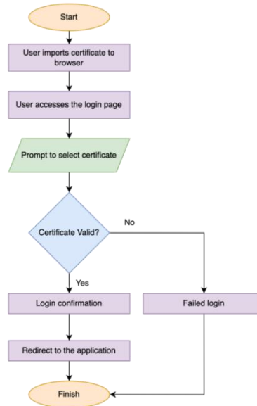
Figure 5. Login flow
