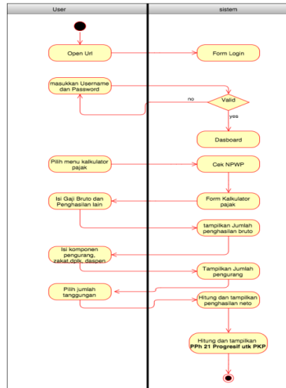
Gambar 1 activity diagram
